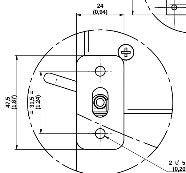
DETAIL B GIMBLE PLATE DETAIL
